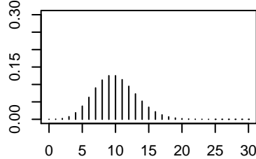
Poisson, \lambda=10.0
