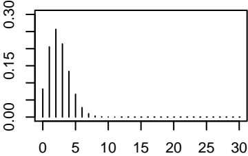
Poisson, \lambda=2.5
