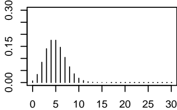
Poisson, \lambda=5.0
